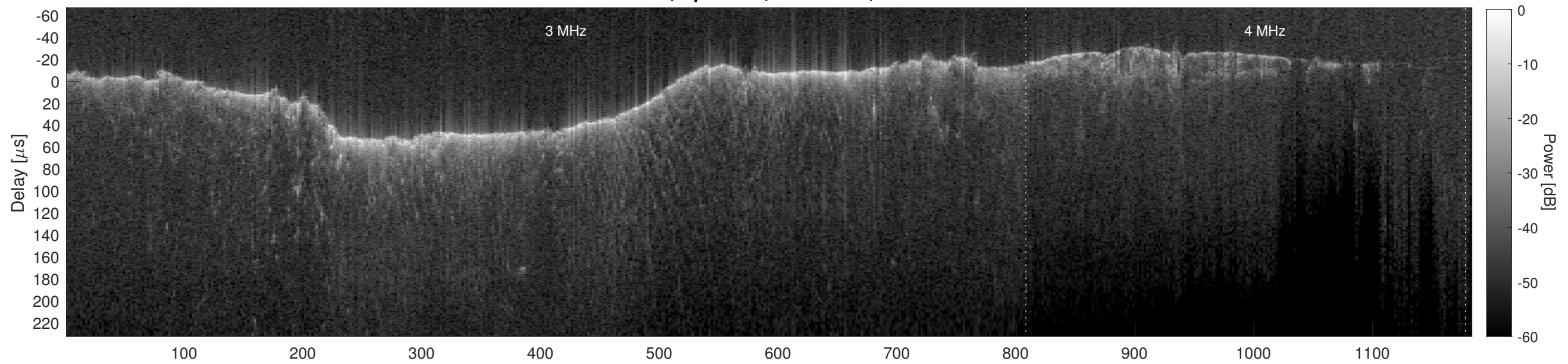
Orbit 21477, Cluttergram
