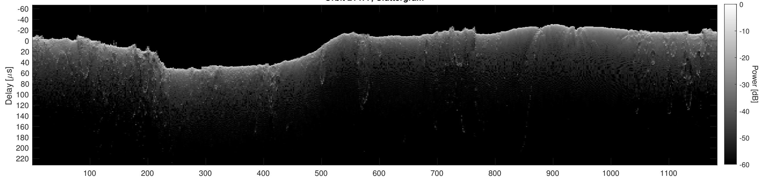
Orbit 21477, Cluttergram
