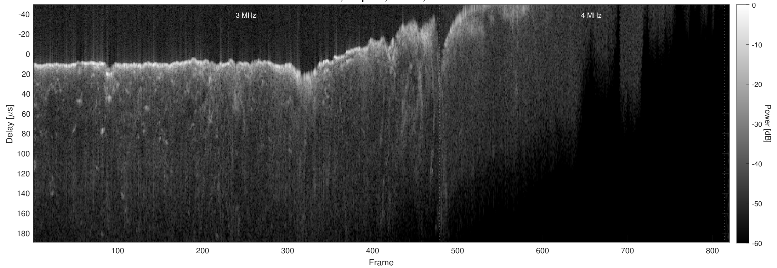
Orbit 21488, Chapman, Window, Channel 2
