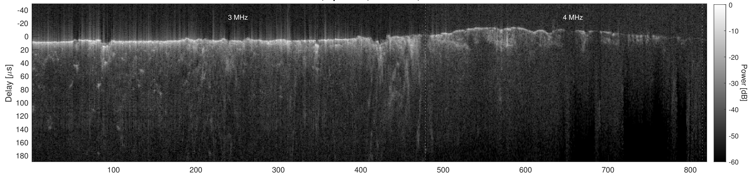
Orbit 21488, Cluttergram
