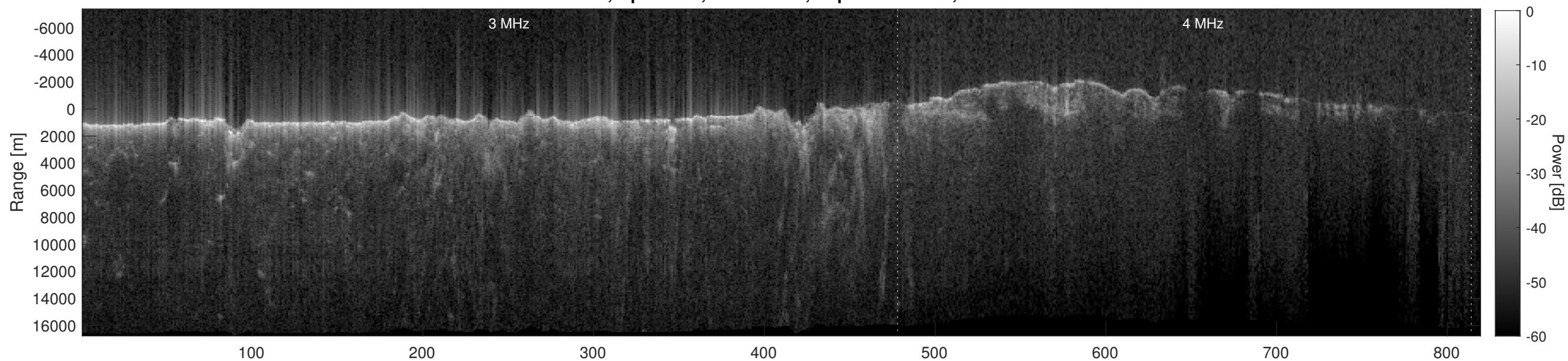
Orbit 21488, Depth-Corrected Cluttergram
