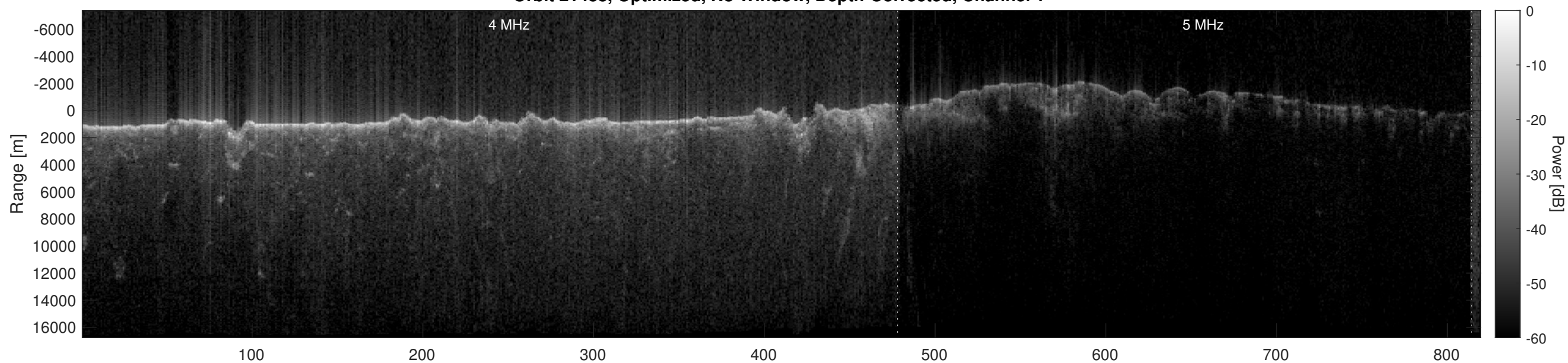
Orbit 21488, Optimized, No Window, Depth-Corrected, Channel 2
