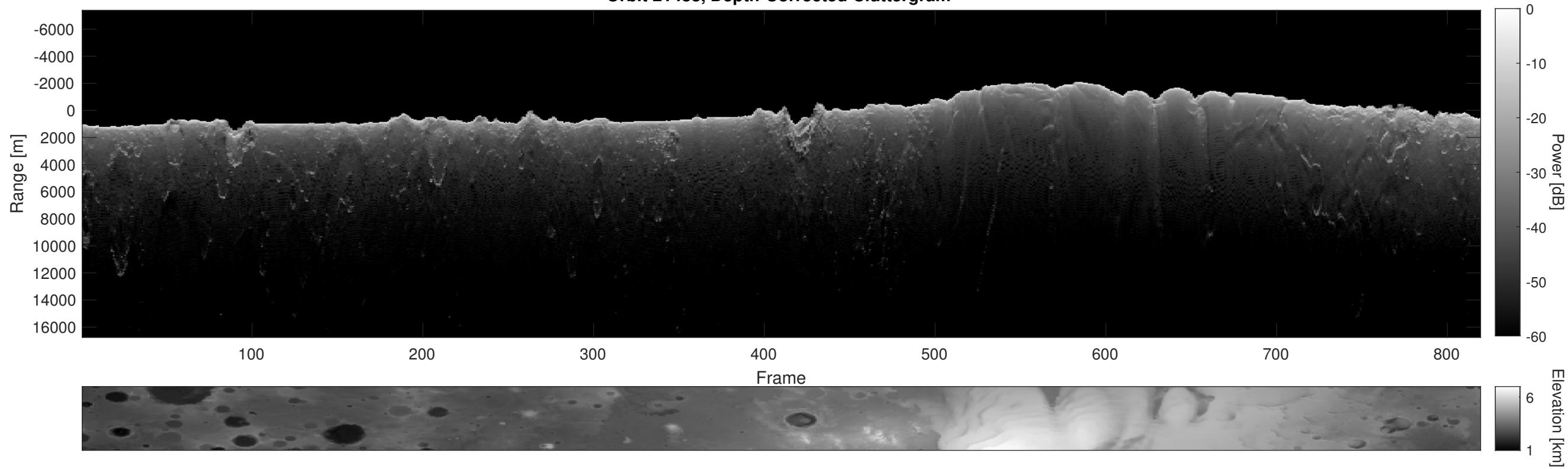
Orbit 21488, Depth-Corrected Cluttergram
