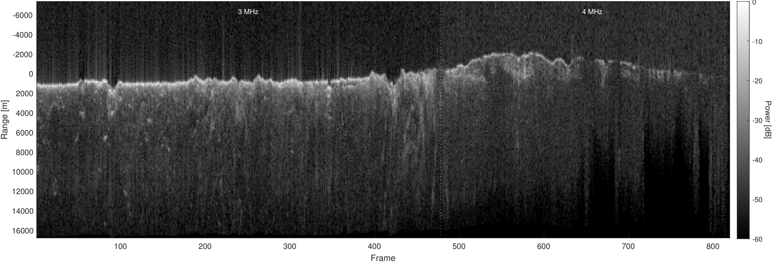
Orbit 21488, Optimized, Window, Depth-Corrected, Channel 2
