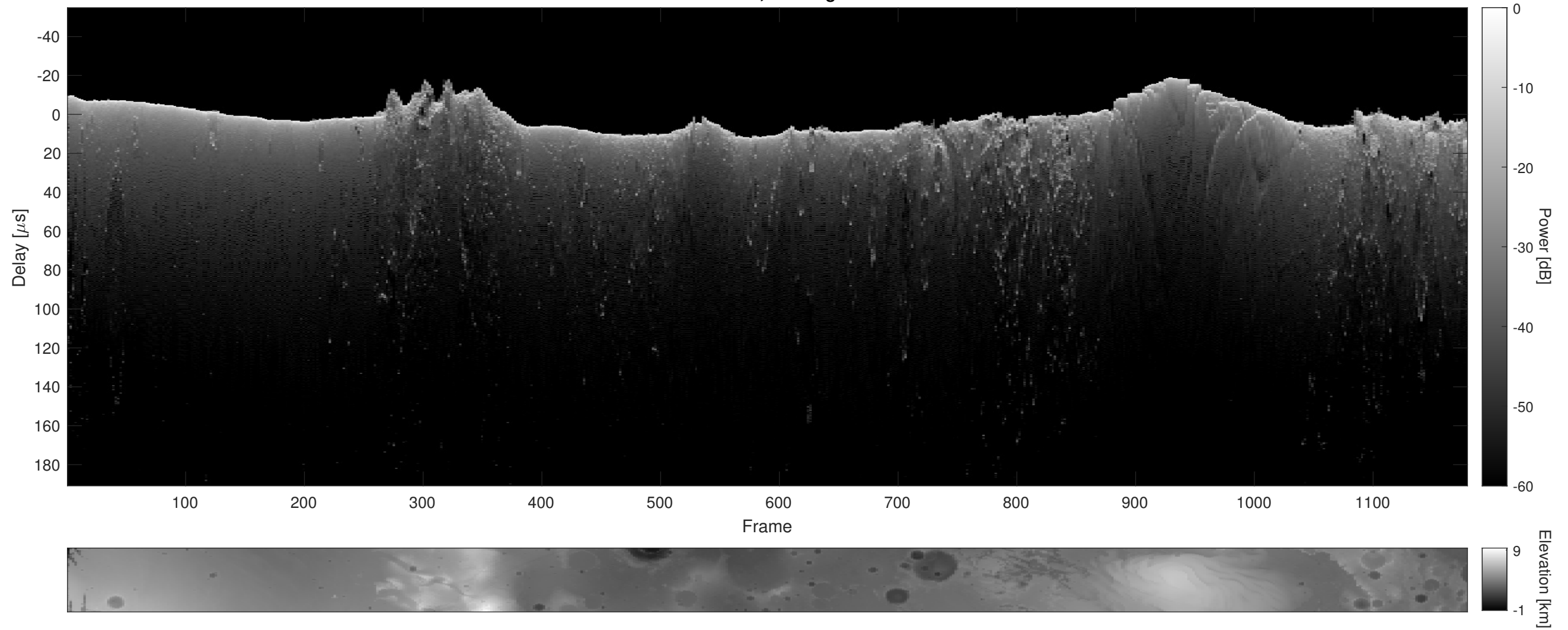
Orbit 21489, Cluttergram
