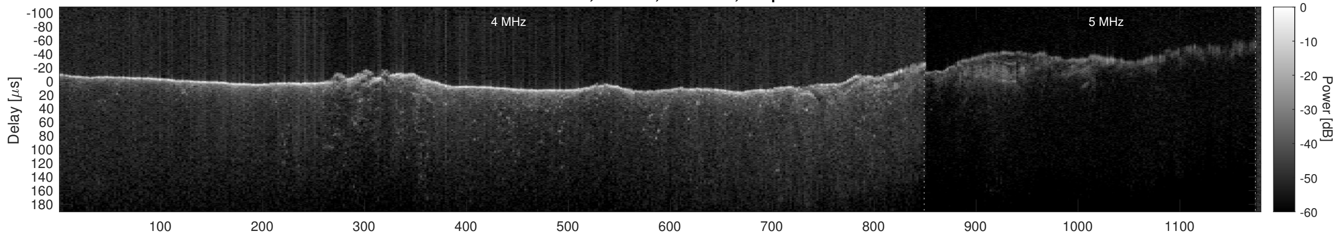
Orbit 21489, Window, Channel 1, Optimized
