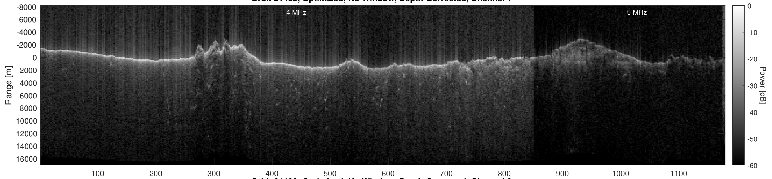
Orbit 21489, Optimized, No Window, Depth-Corrected, Channel 2
