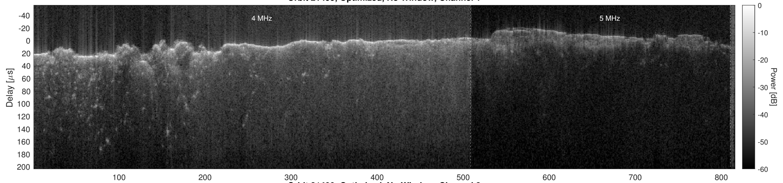
Orbit 21499, Optimized, No Window, Channel 2
