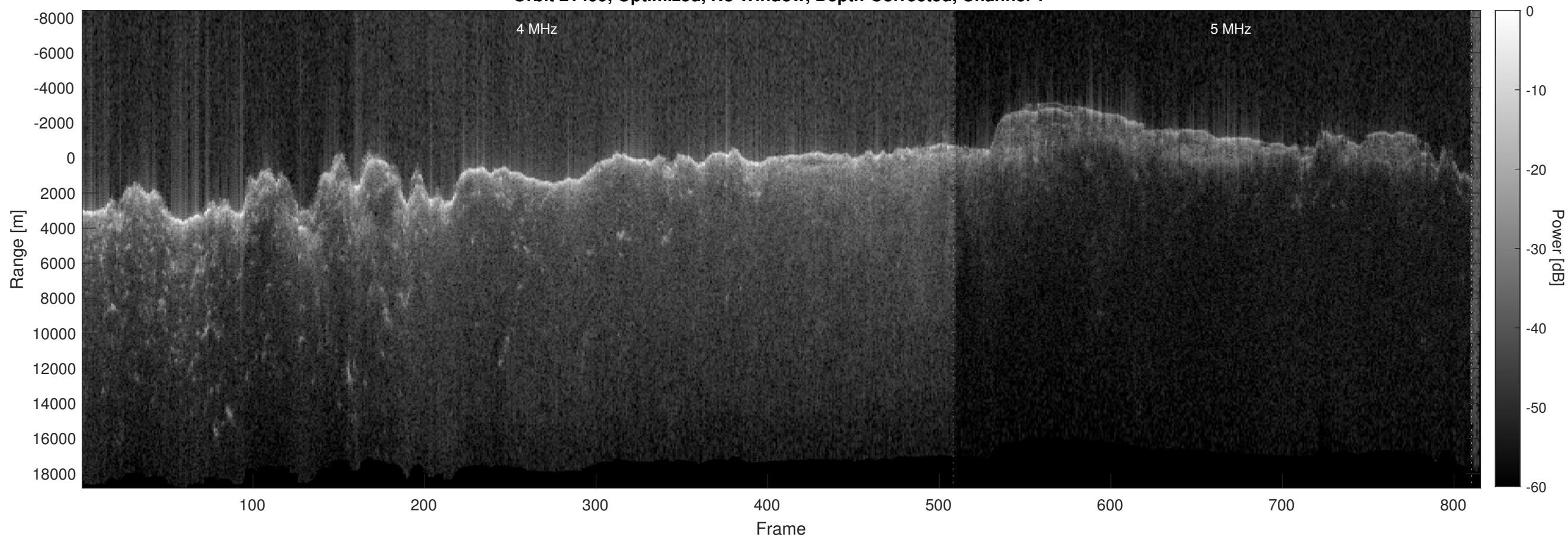
Orbit 21499, Optimized, No Window, Depth-Corrected, Channel 2
