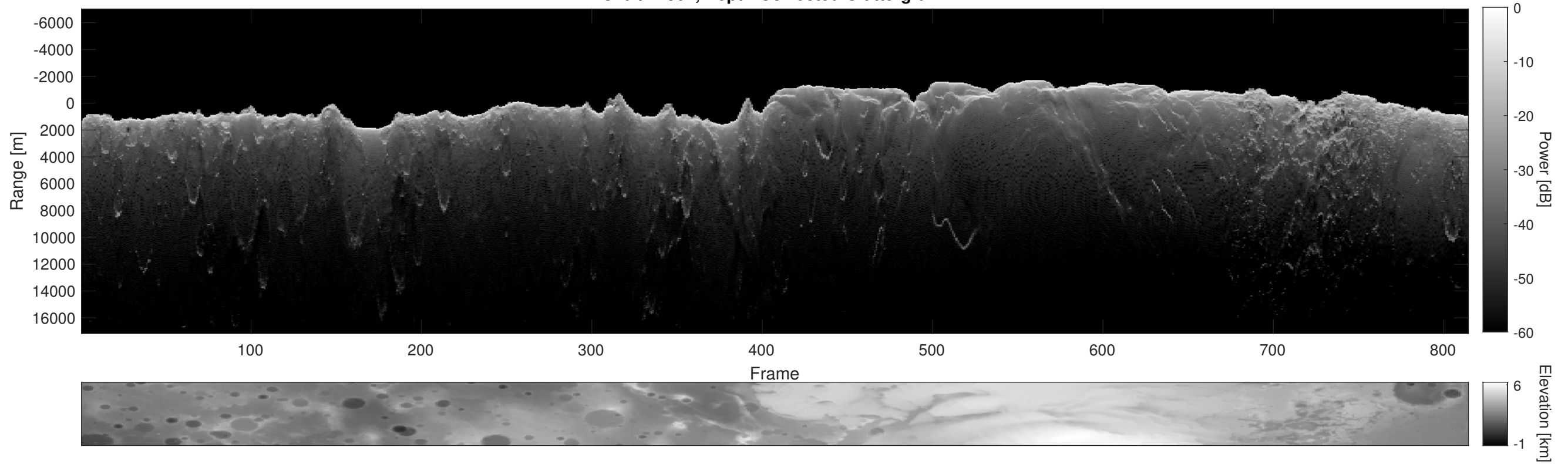
Orbit 21501, Depth-Corrected Cluttergram
