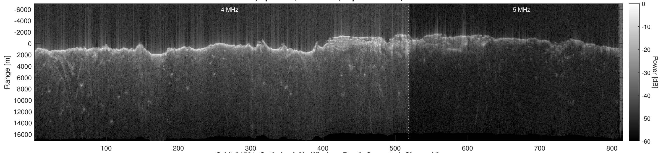
Orbit 21501, Optimized, No Window, Depth-Corrected, Channel 2
