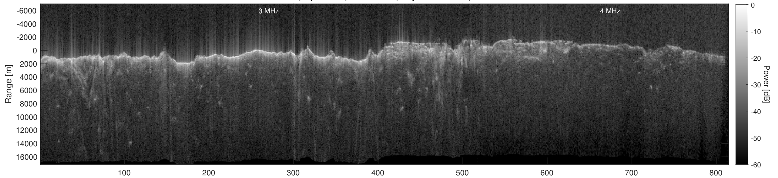
Orbit 21501, Depth-Corrected Cluttergram
