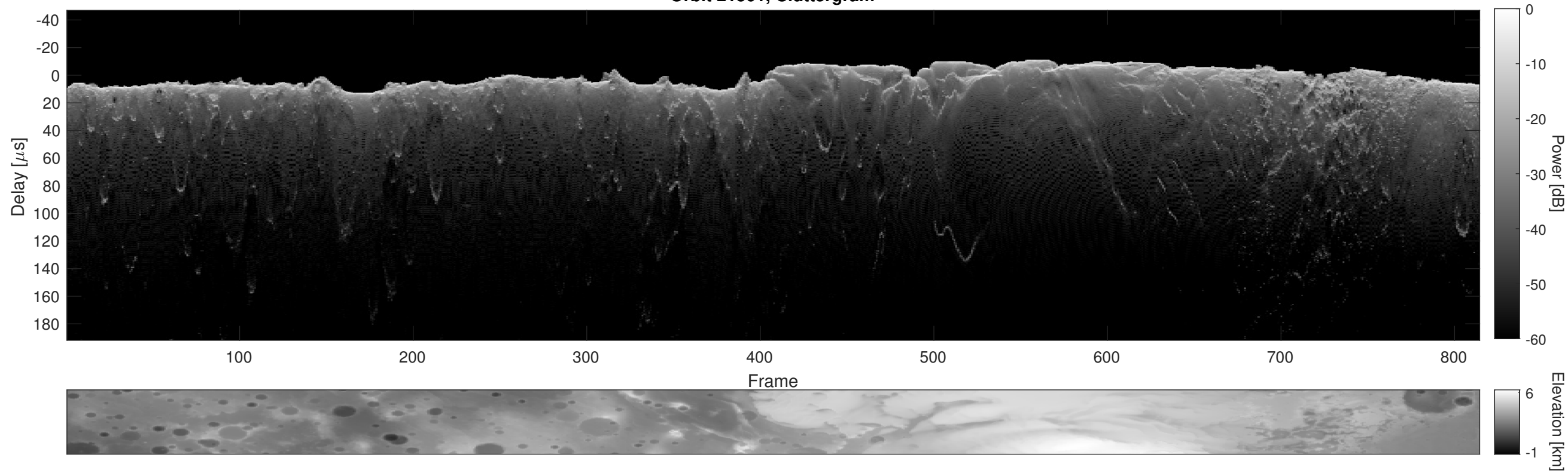
Orbit 21501, Cluttergram
