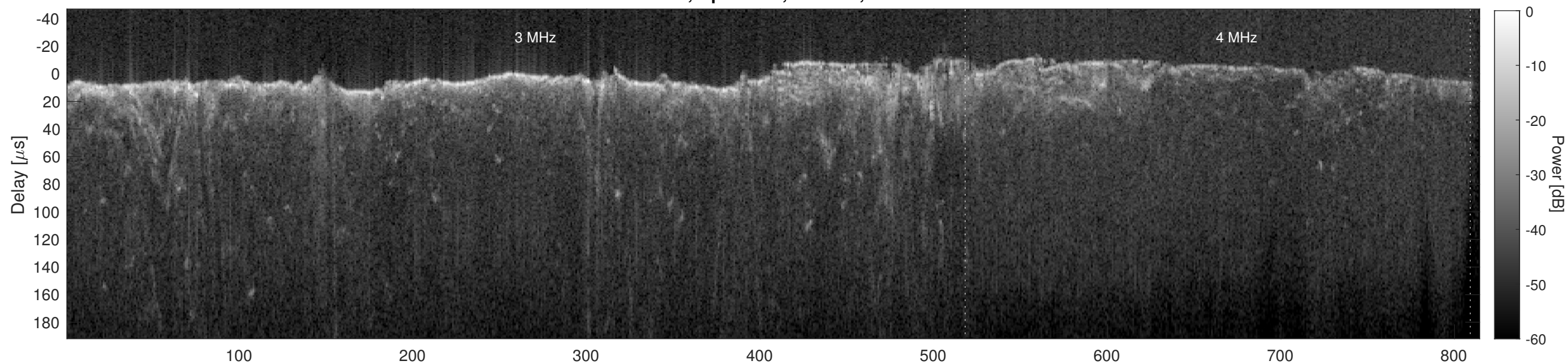
Orbit 21501, Cluttergram
