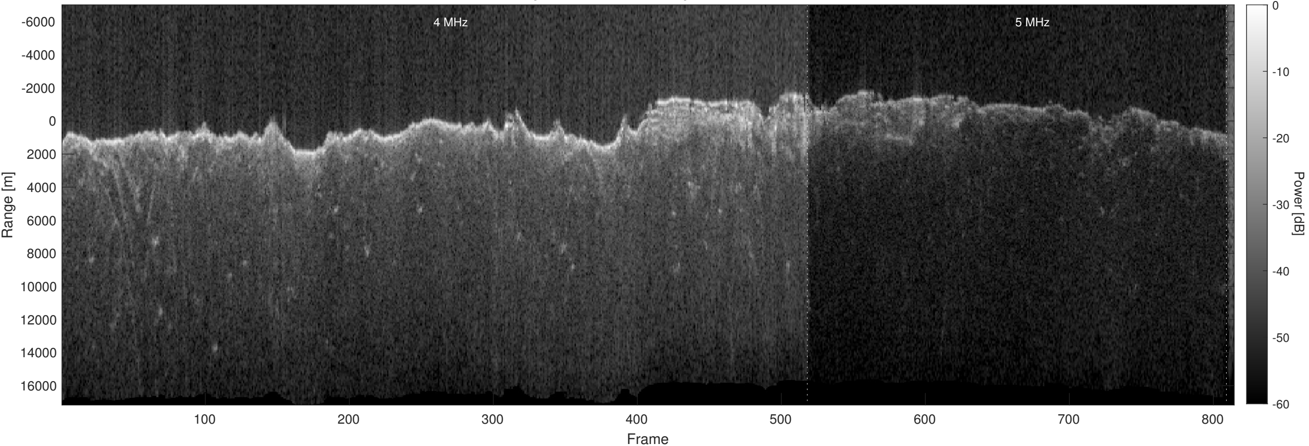
Orbit 21501, Optimized, Window, Depth-Corrected, Channel 2
