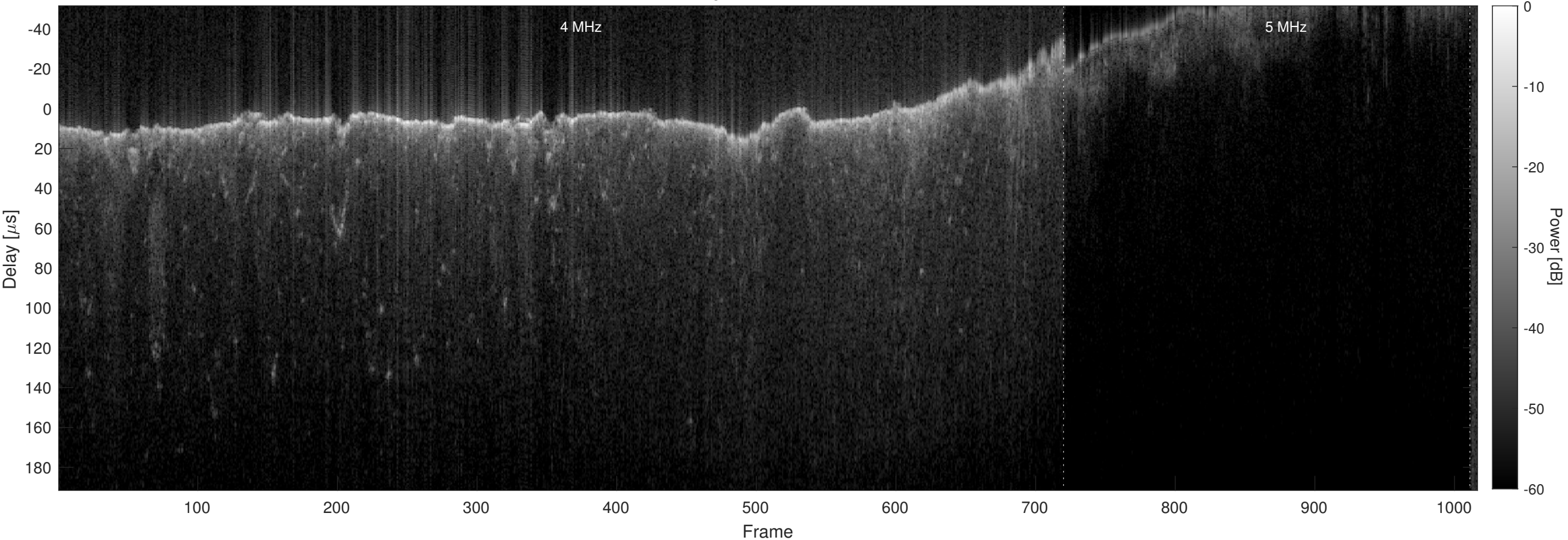
Orbit 21502, Chapman, No Window, Channel 2
