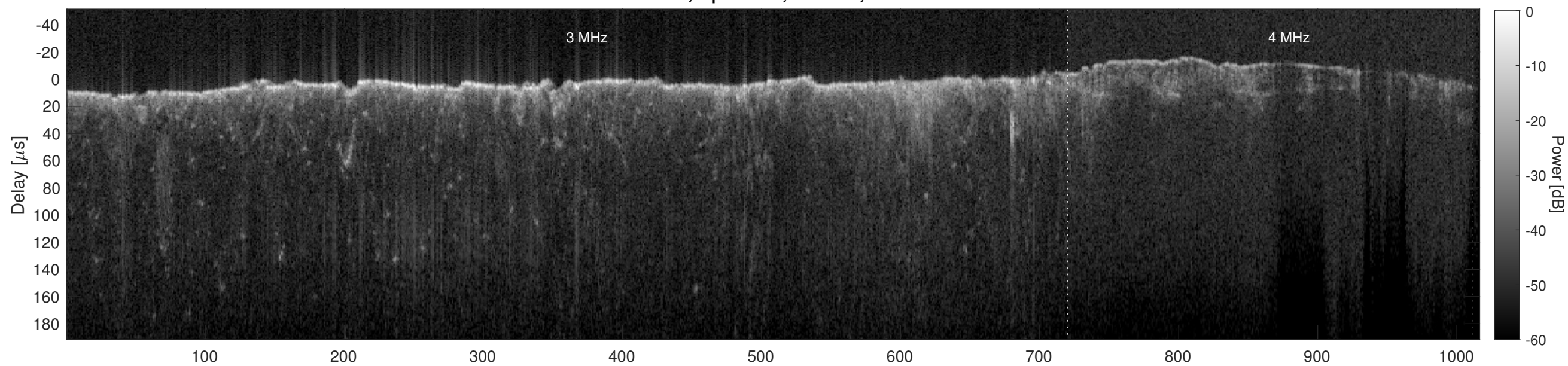
Orbit 21502, Cluttergram
