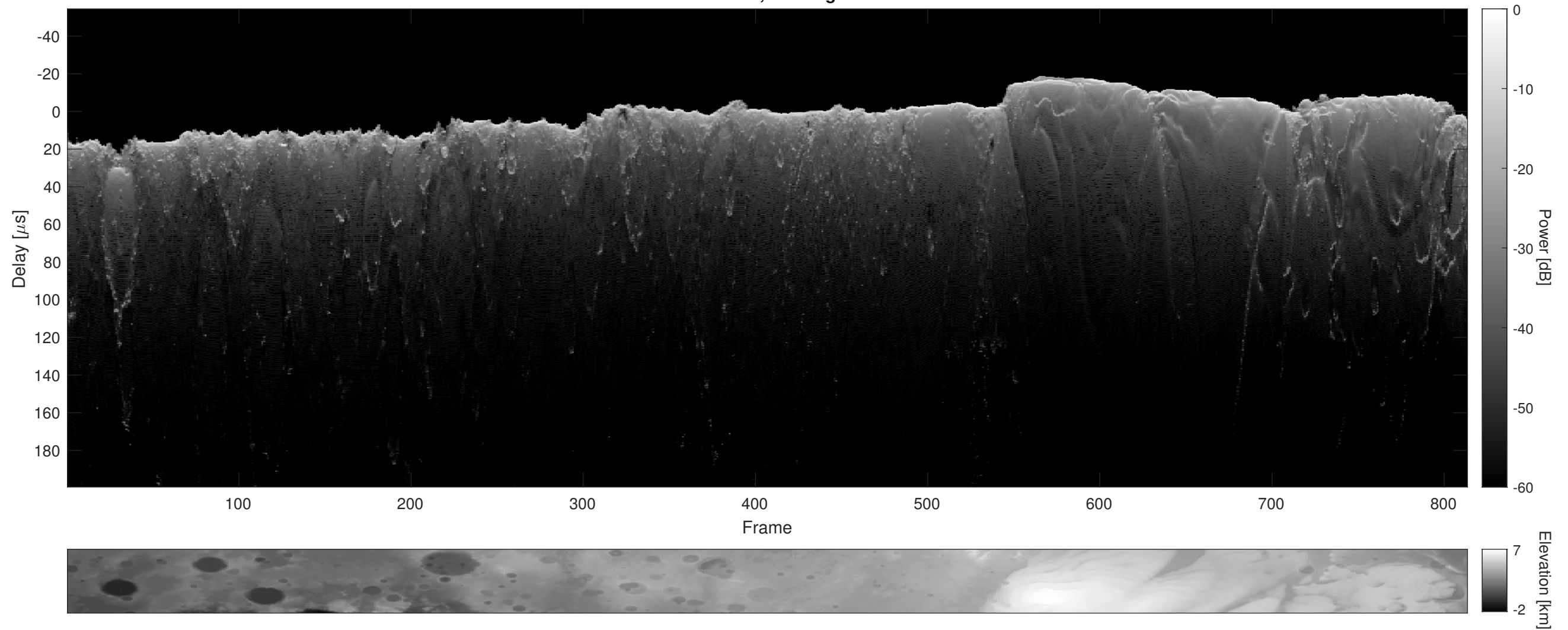
Orbit 21506, Cluttergram
