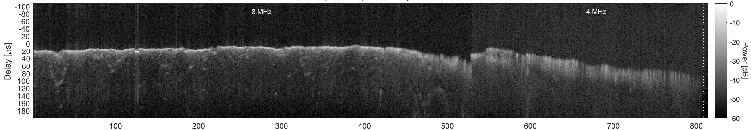
Orbit 21506, Window, Channel 2, Chapman
