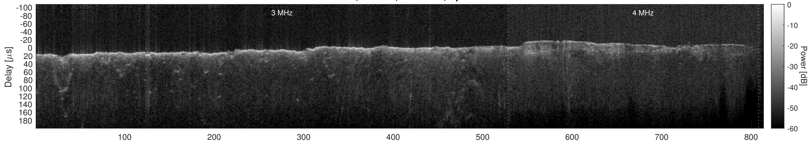
Orbit 21506, Cluttergram
