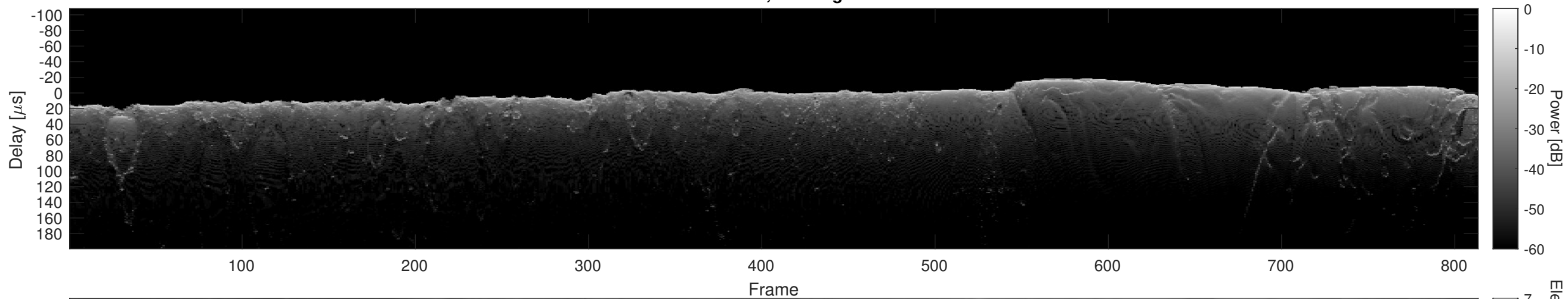
Orbit 21506, Cluttergram
