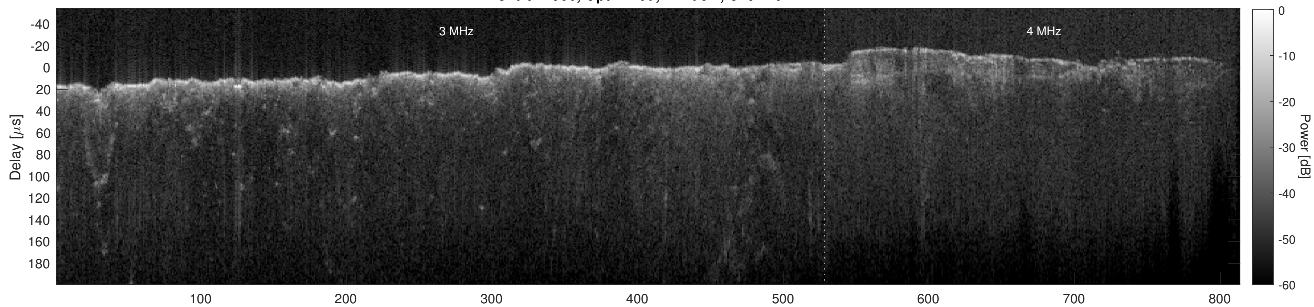
Orbit 21506, Cluttergram
