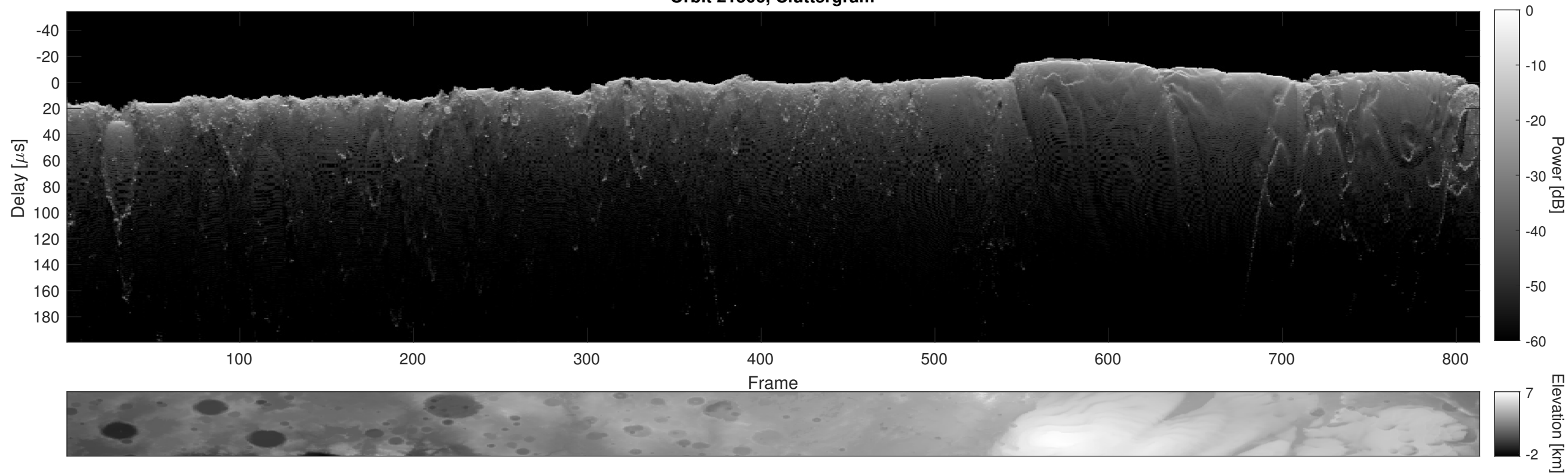
Orbit 21506, Cluttergram
