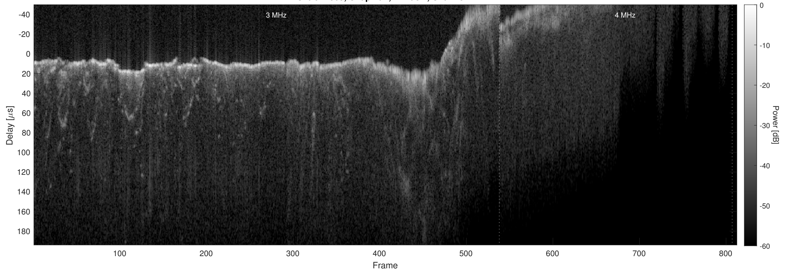
Orbit 21509, Chapman, Window, Channel 2
