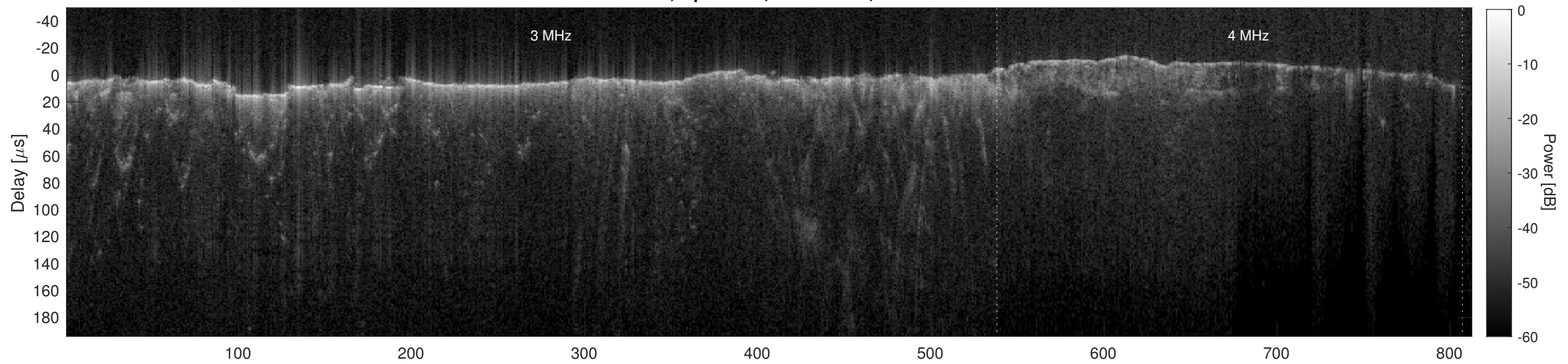
Orbit 21509, Cluttergram
