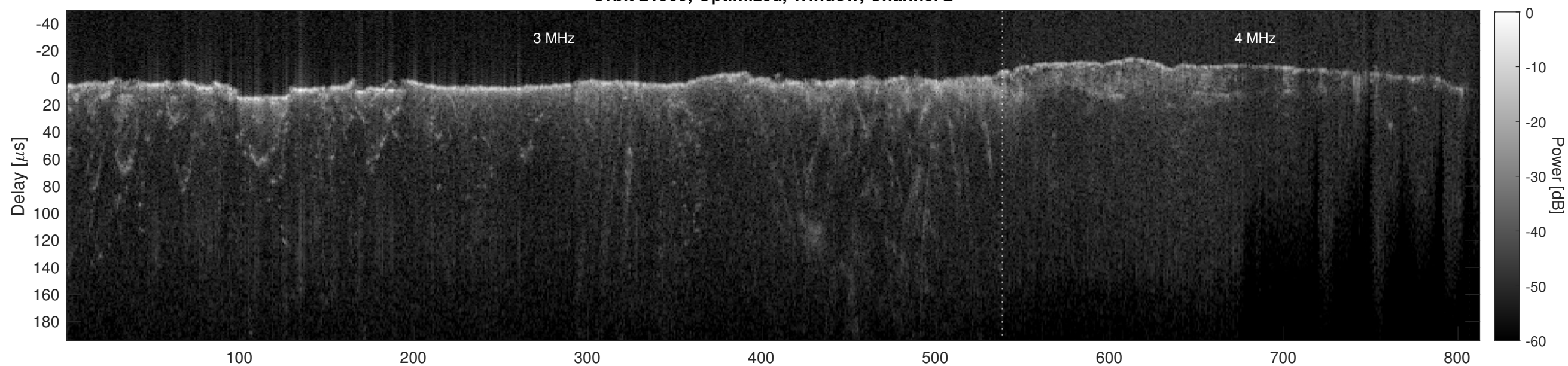
Orbit 21509, Cluttergram
