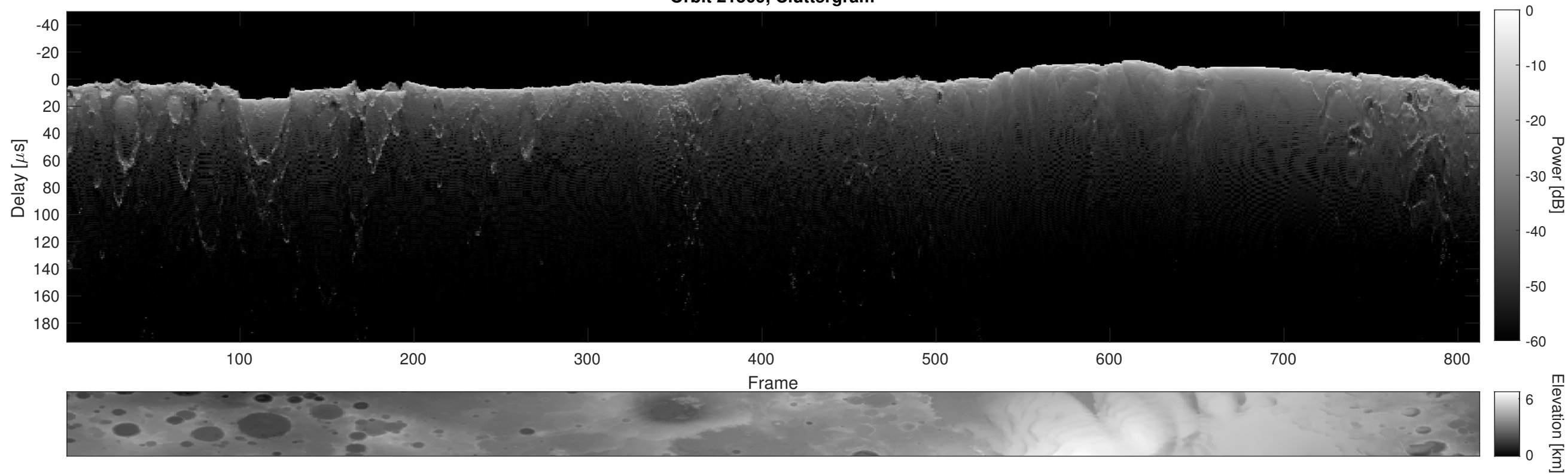
Orbit 21509, Cluttergram
