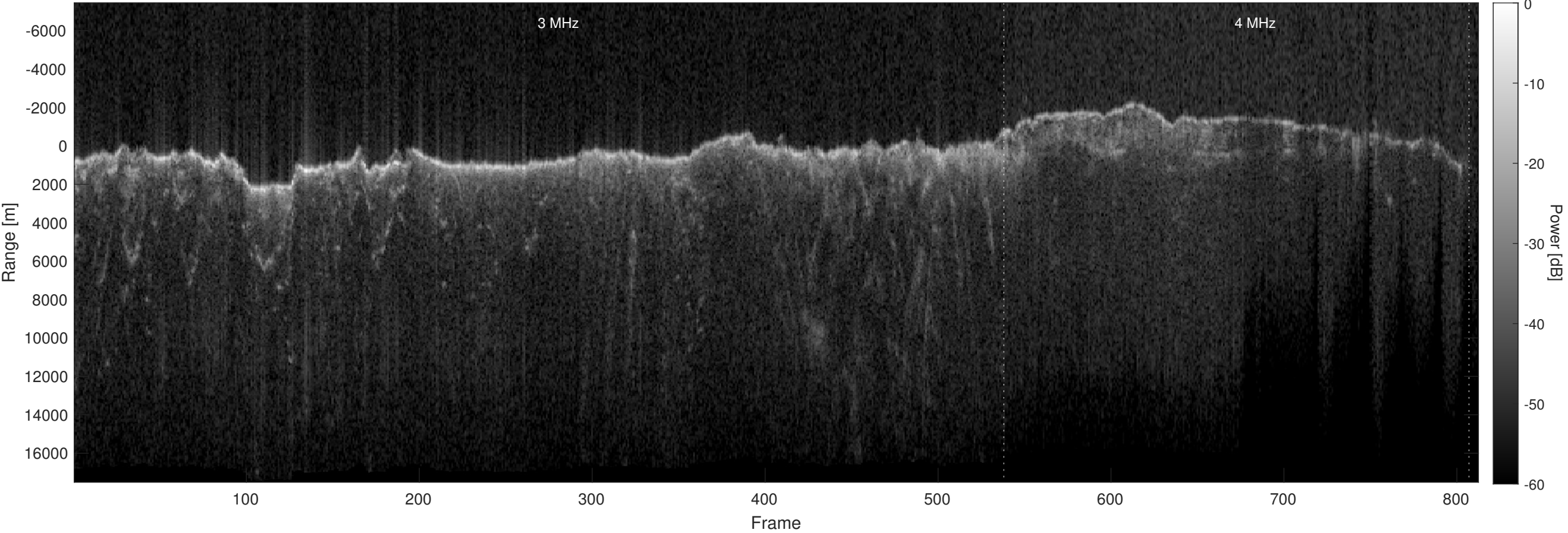
Orbit 21509, Optimized, Window, Depth-Corrected, Channel 2
