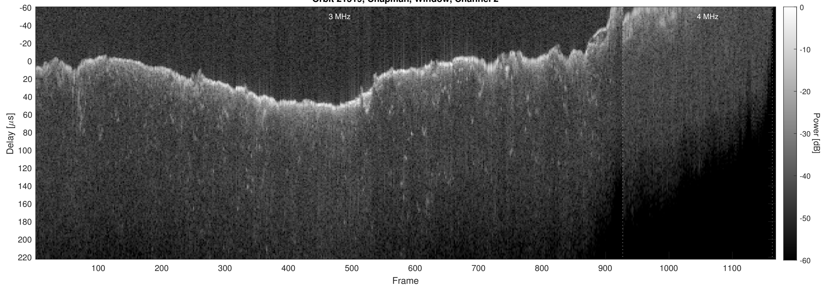
Orbit 21519, Chapman, Window, Channel 2
