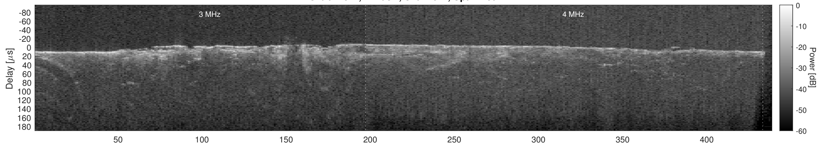
Orbit 21522, Cluttergram
