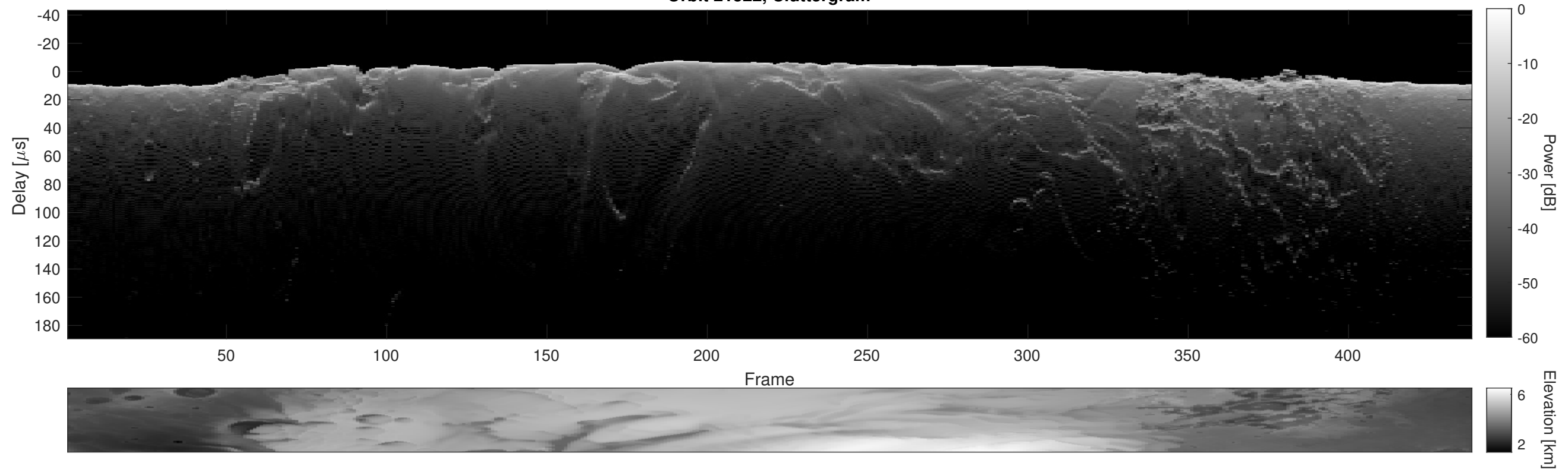
Orbit 21522, Cluttergram
