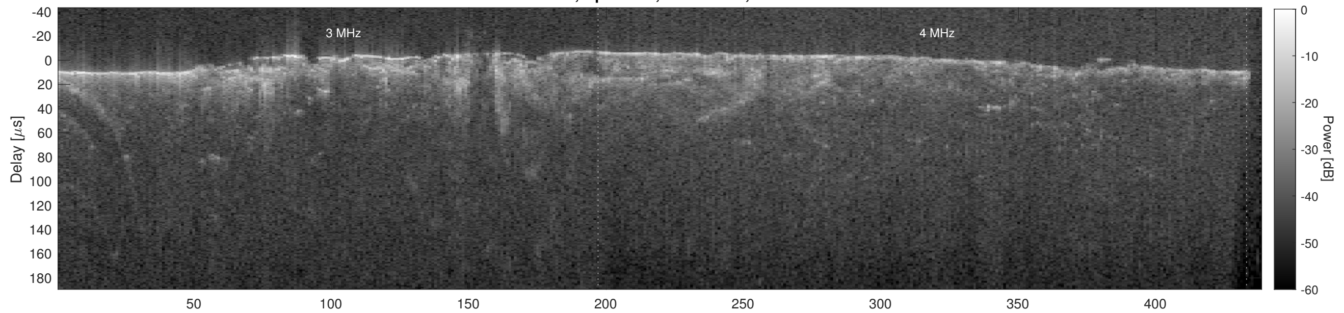
Orbit 21522, Cluttergram
