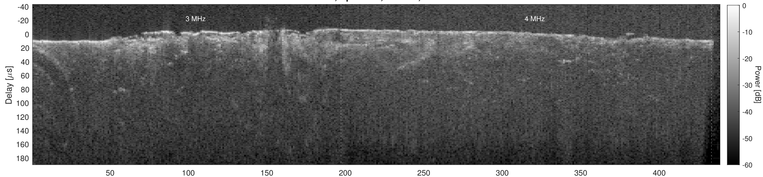
Orbit 21522, Cluttergram
