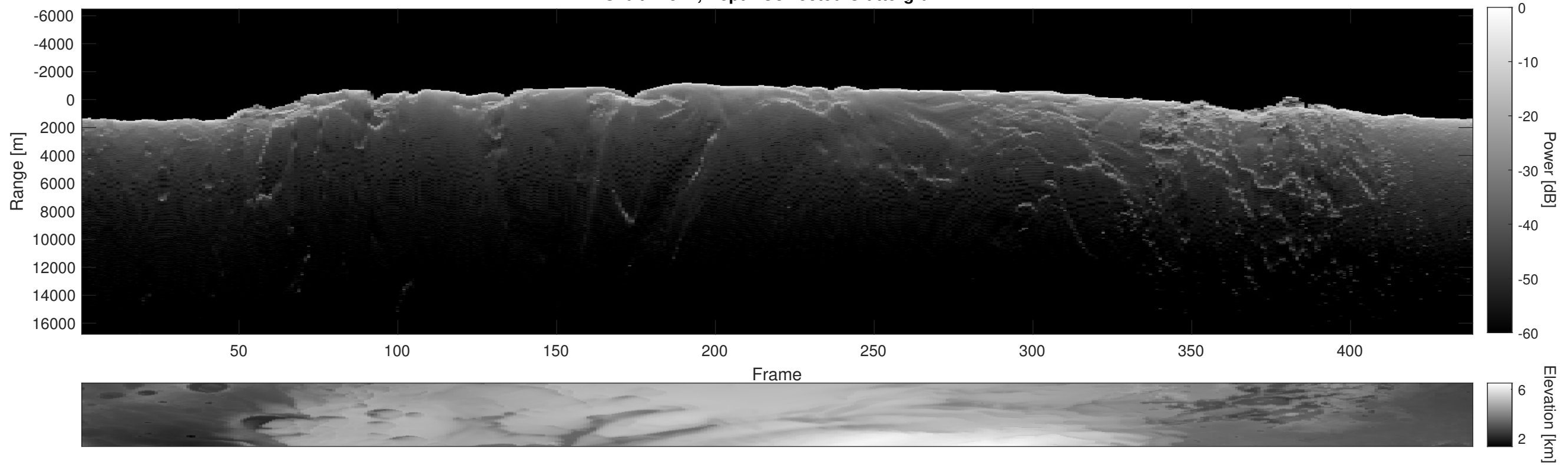
Orbit 21522, Depth-Corrected Cluttergram
