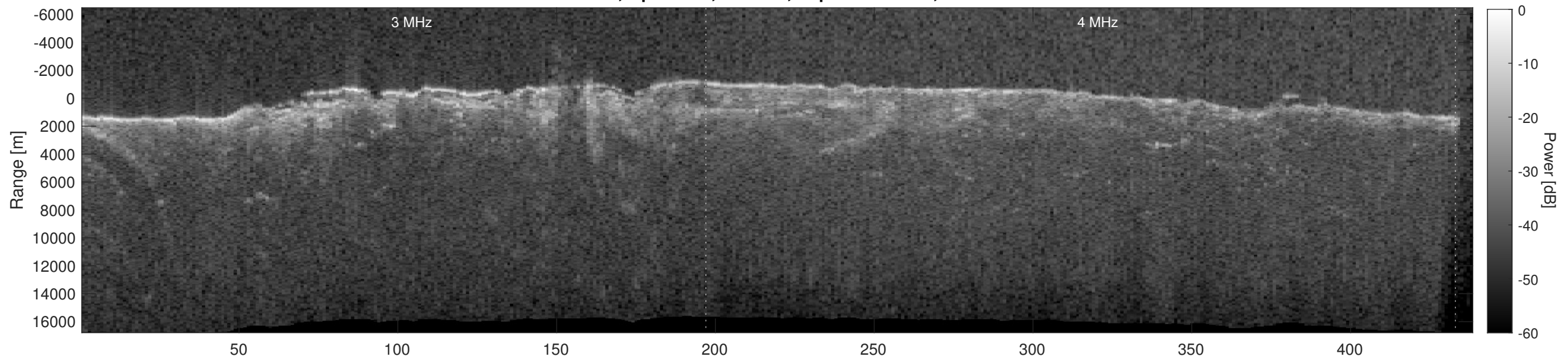
Orbit 21522, Depth-Corrected Cluttergram
