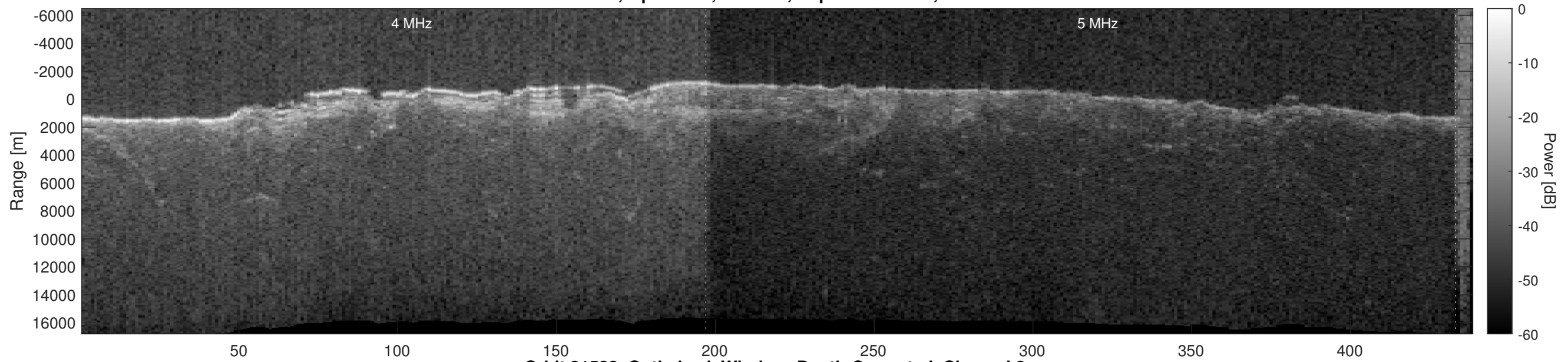
Orbit 21522, Optimized, Window, Depth-Corrected, Channel 2
