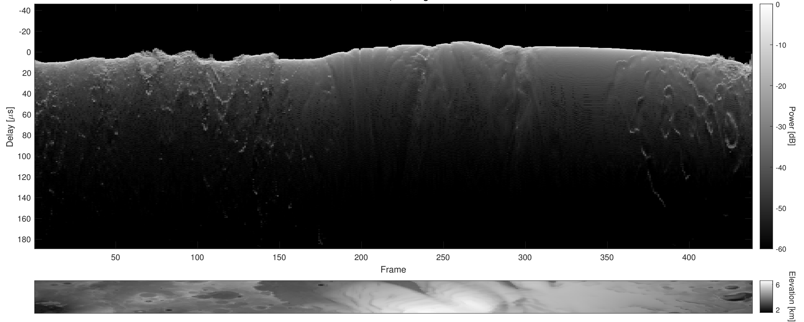
Orbit 21523, Cluttergram
