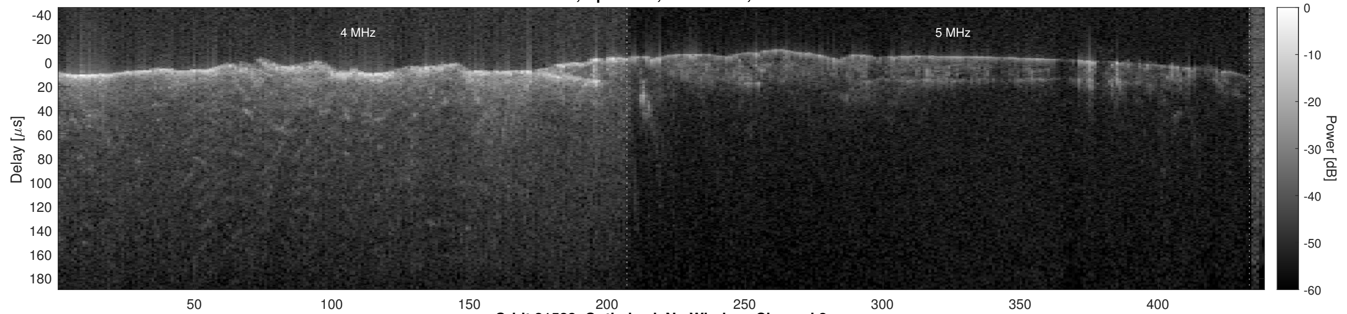
Orbit 21523, Optimized, No Window, Channel 2
