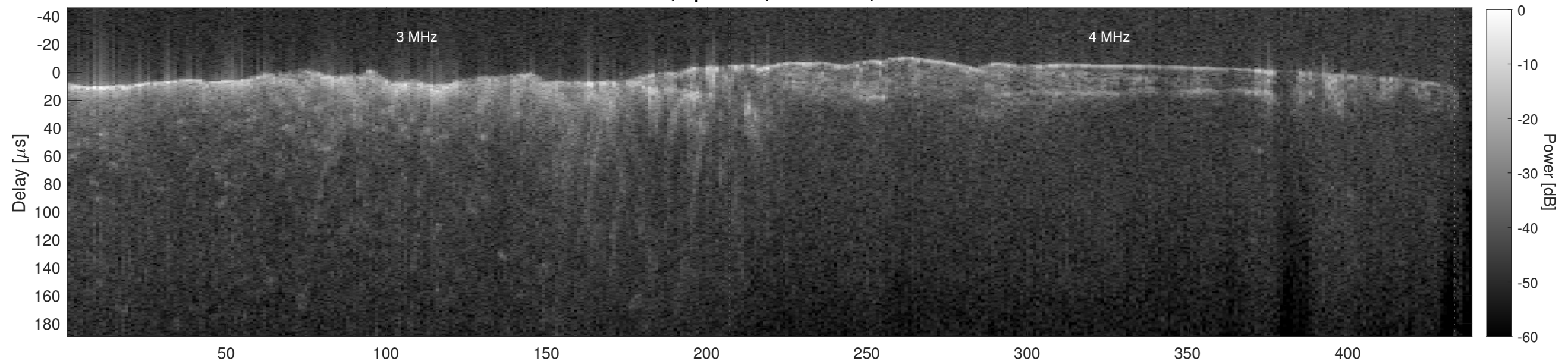
Orbit 21523, Cluttergram
