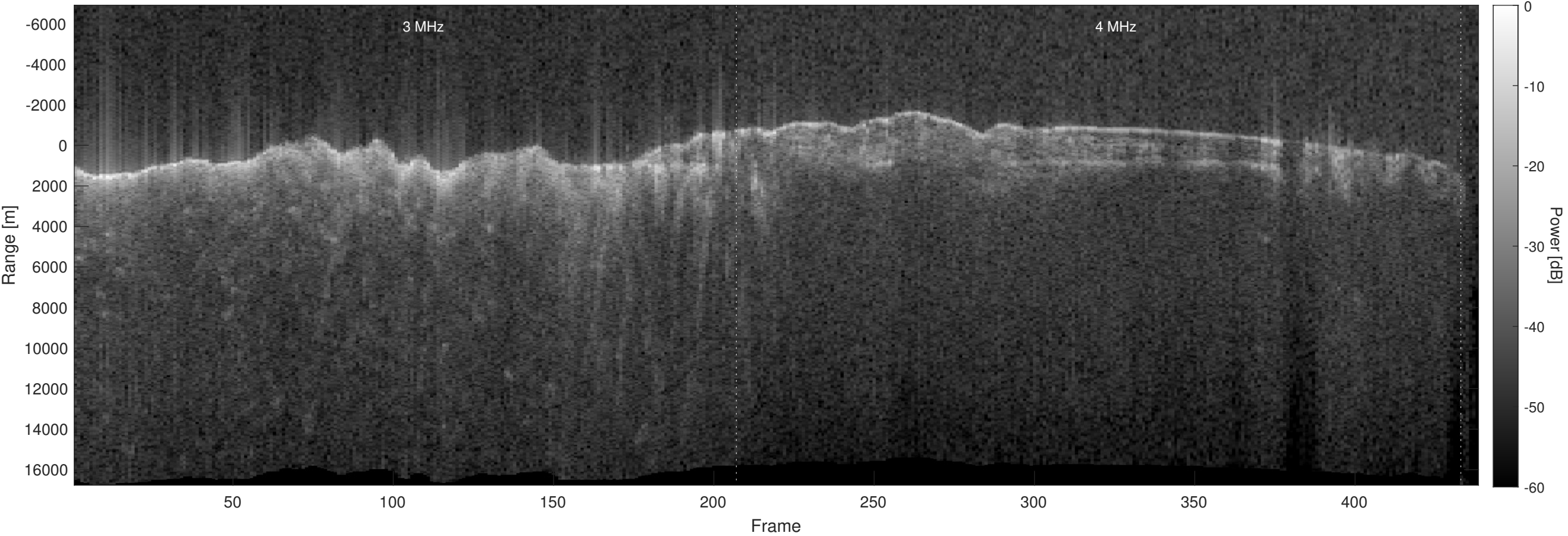
Orbit 21523, Optimized, No Window, Depth-Corrected, Channel 2
