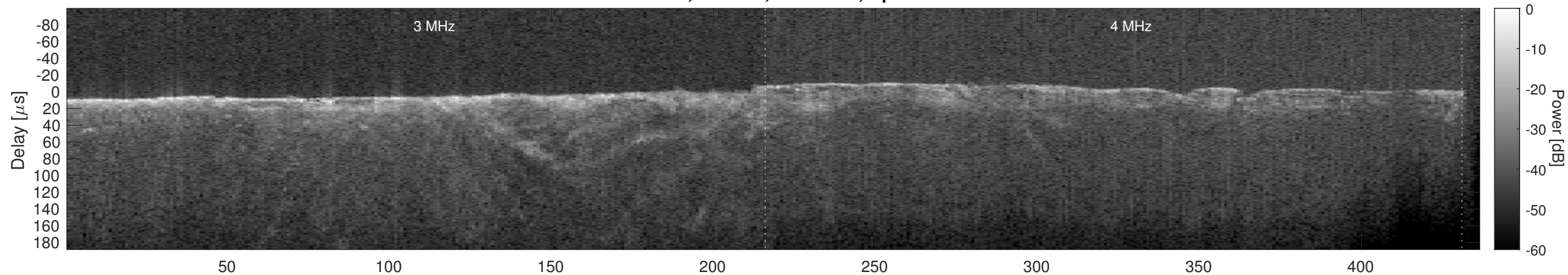
Orbit 21527, Cluttergram
