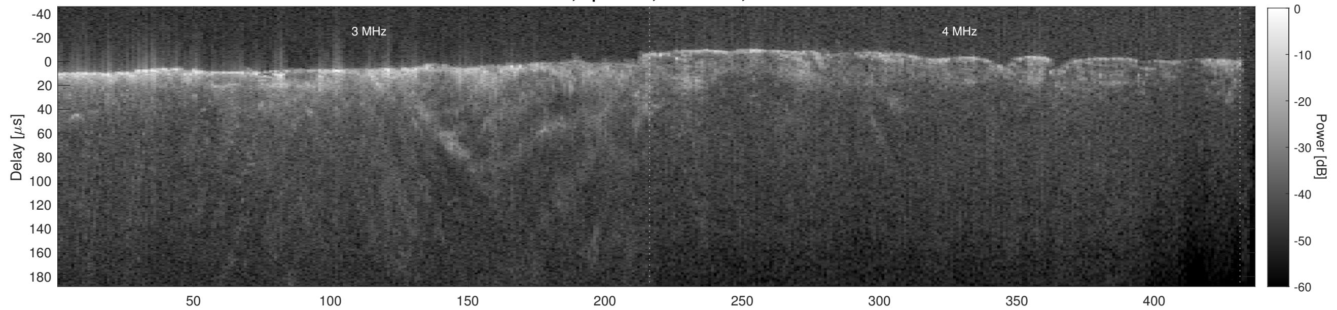
Orbit 21527, Cluttergram
