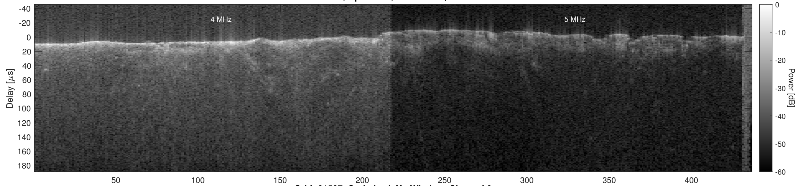
Orbit 21527, Optimized, No Window, Channel 2
