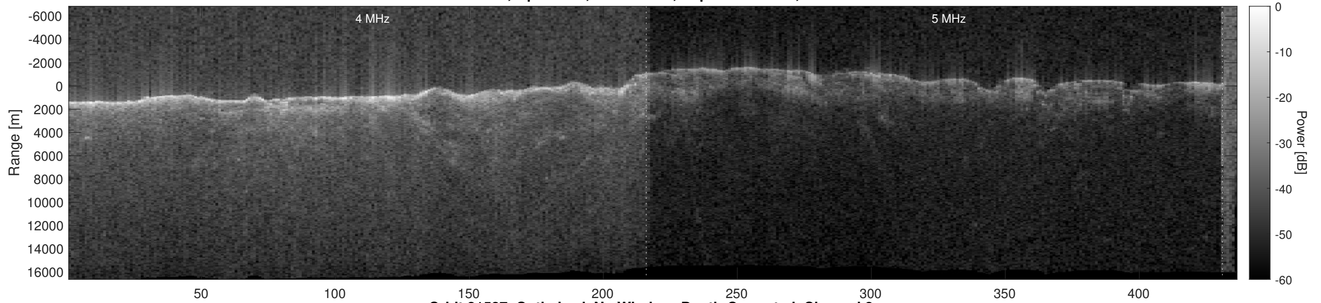
Orbit 21527, Optimized, No Window, Depth-Corrected, Channel 2
