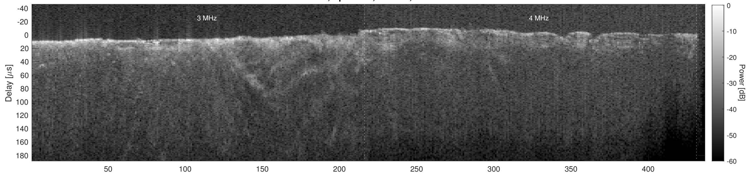
Orbit 21527, Cluttergram
