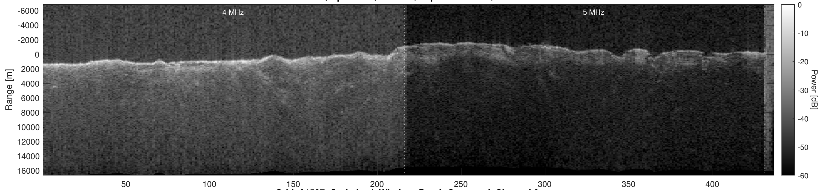
Orbit 21527, Optimized, Window, Depth-Corrected, Channel 2
