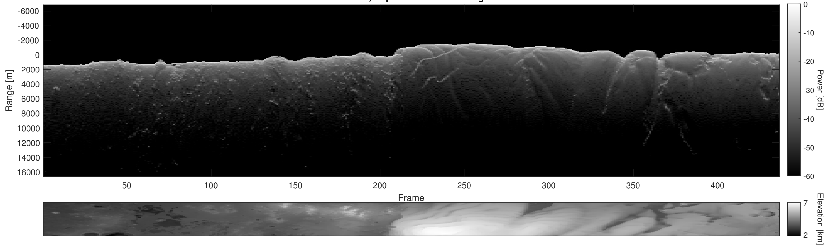
Orbit 21527, Depth-Corrected Cluttergram
