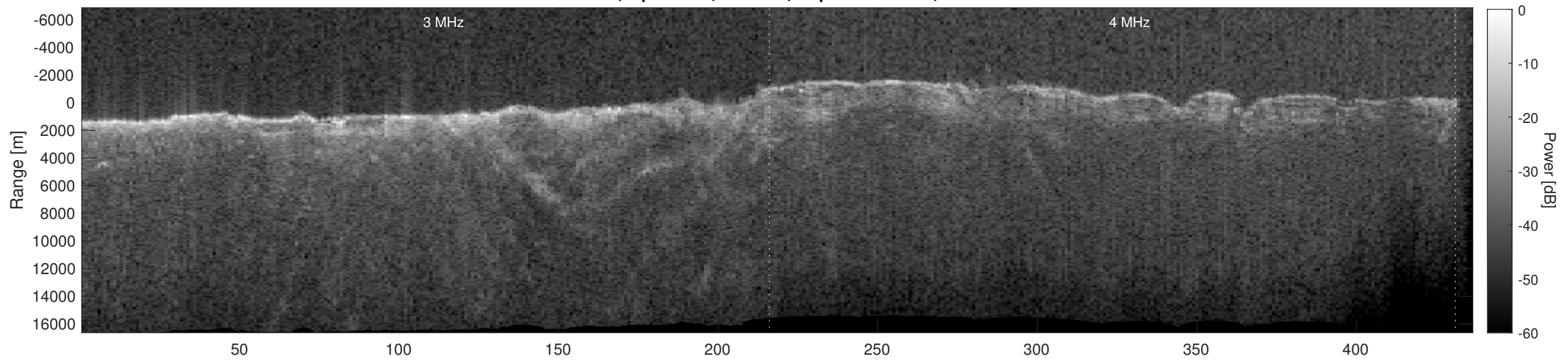
Orbit 21527, Depth-Corrected Cluttergram
