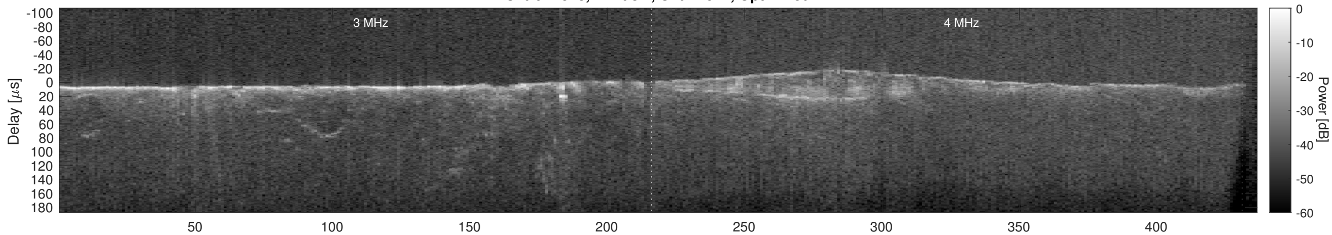
Orbit 21528, Cluttergram
