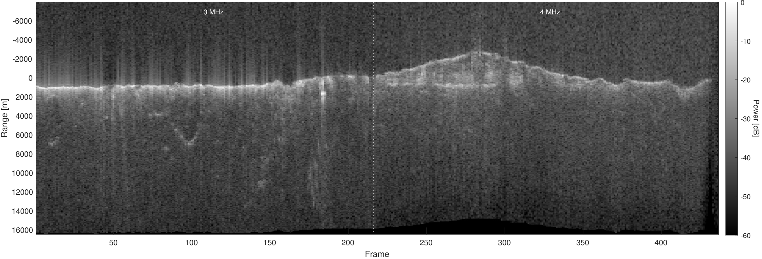
Orbit 21528, Optimized, No Window, Depth-Corrected, Channel 2
