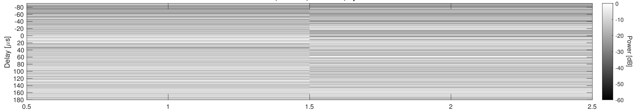
Orbit 21529, Cluttergram
