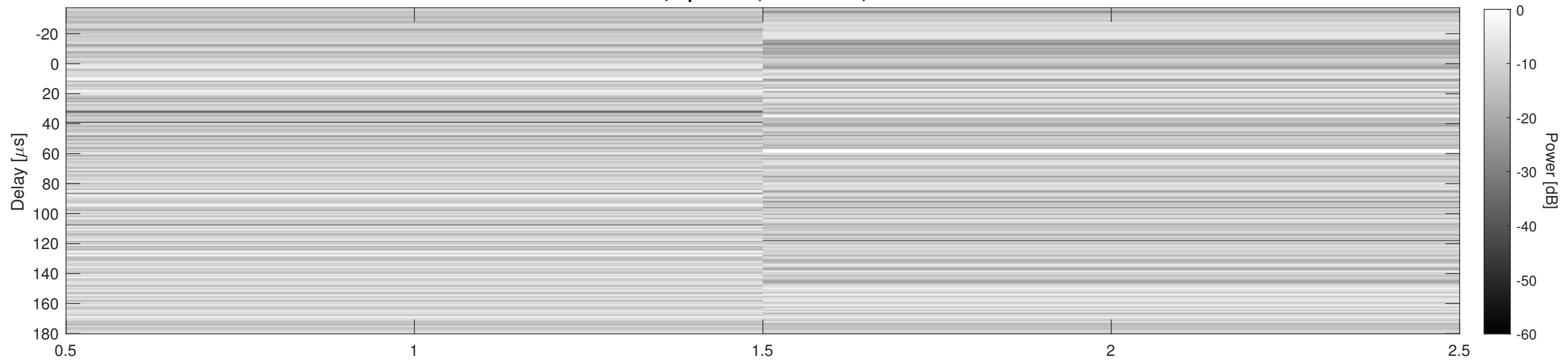
Orbit 21529, Cluttergram
