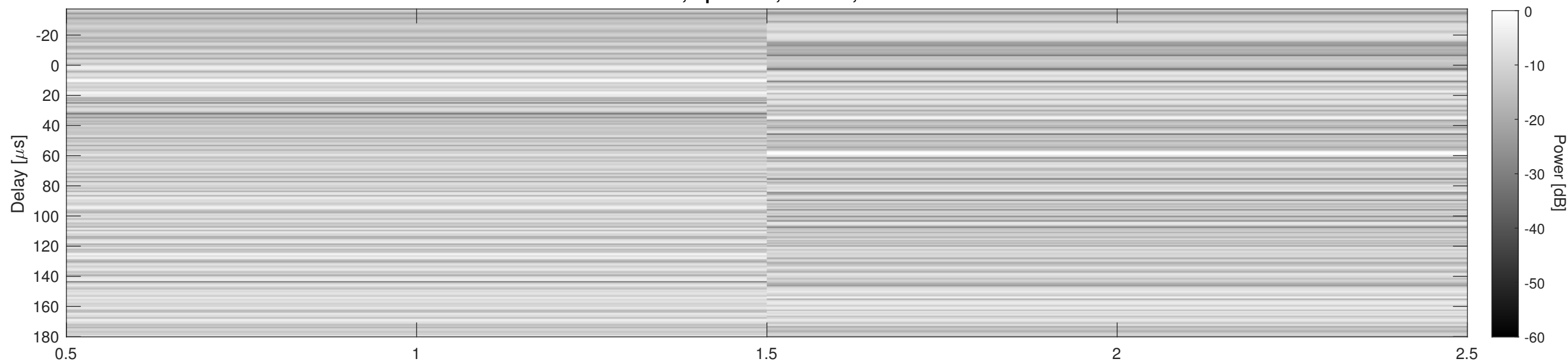
Orbit 21529, Cluttergram
