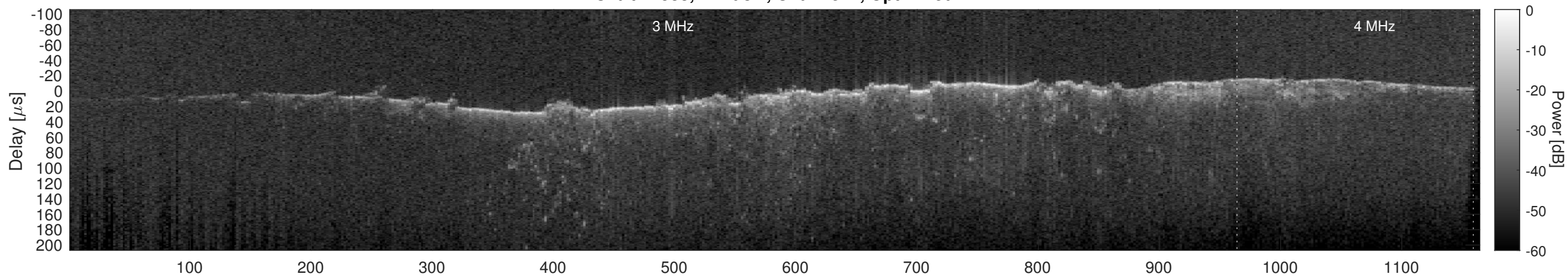
Orbit 21533, Cluttergram
