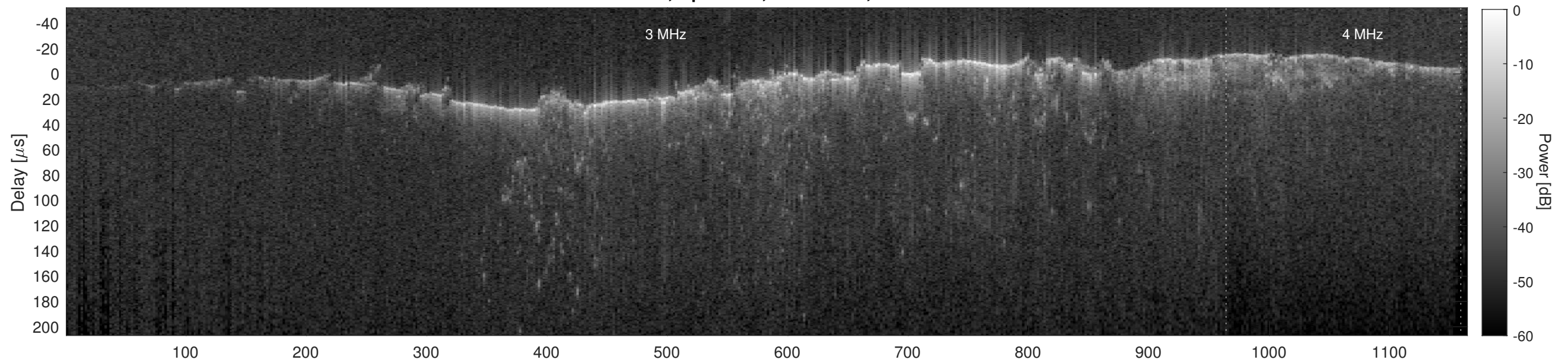
Orbit 21533, Cluttergram
