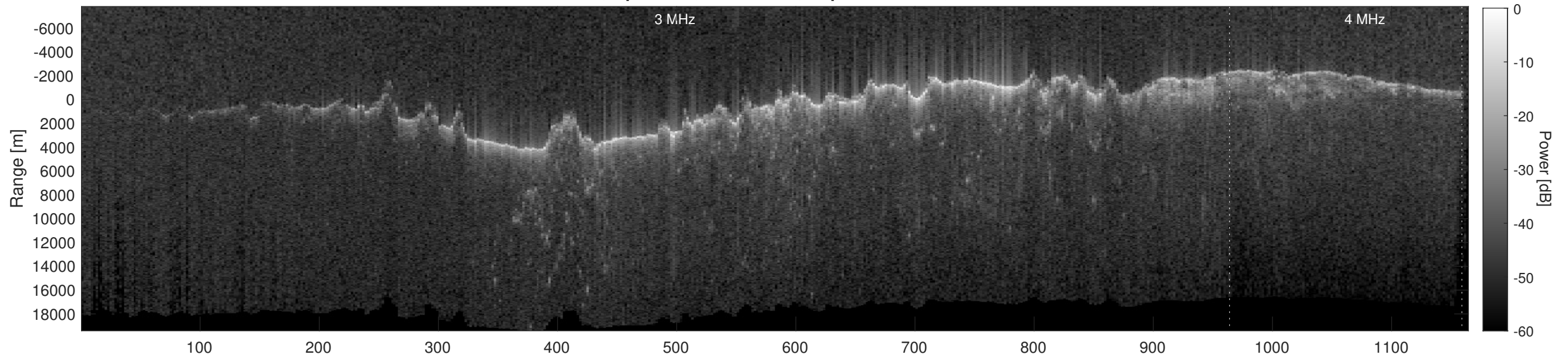
Orbit 21533, Depth-Corrected Cluttergram
