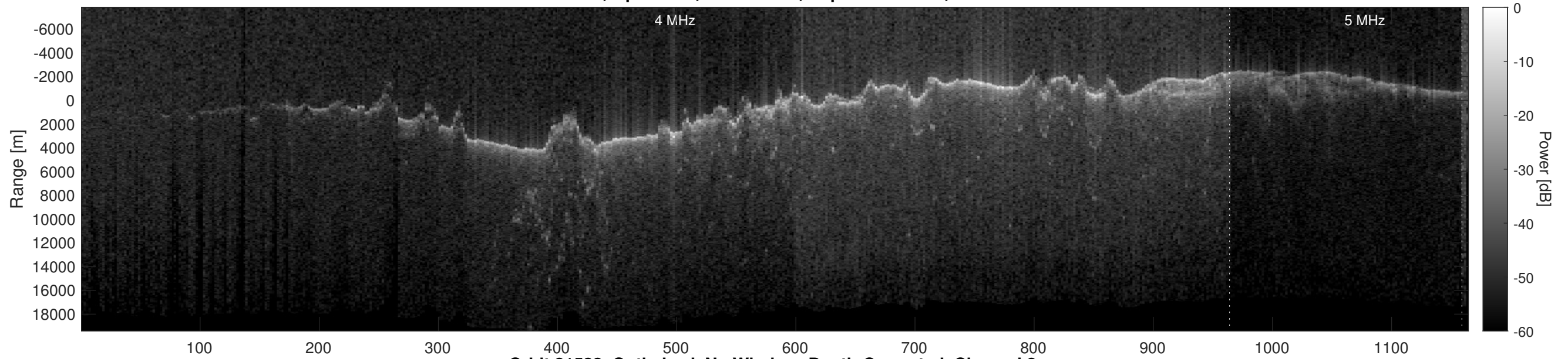
Orbit 21533, Optimized, No Window, Depth-Corrected, Channel 2
