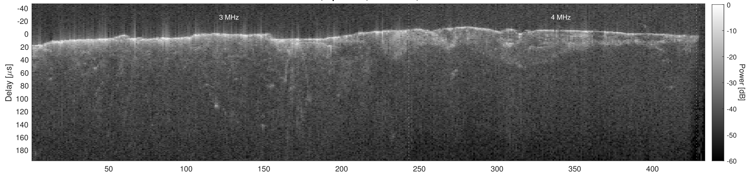
Orbit 21537, Cluttergram
