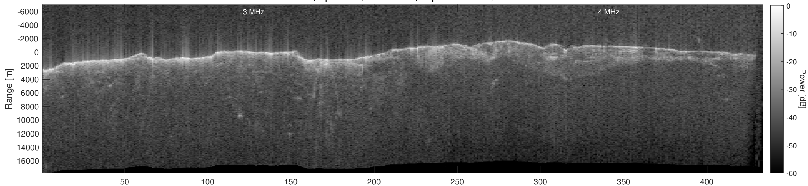
Orbit 21537, Depth-Corrected Cluttergram
