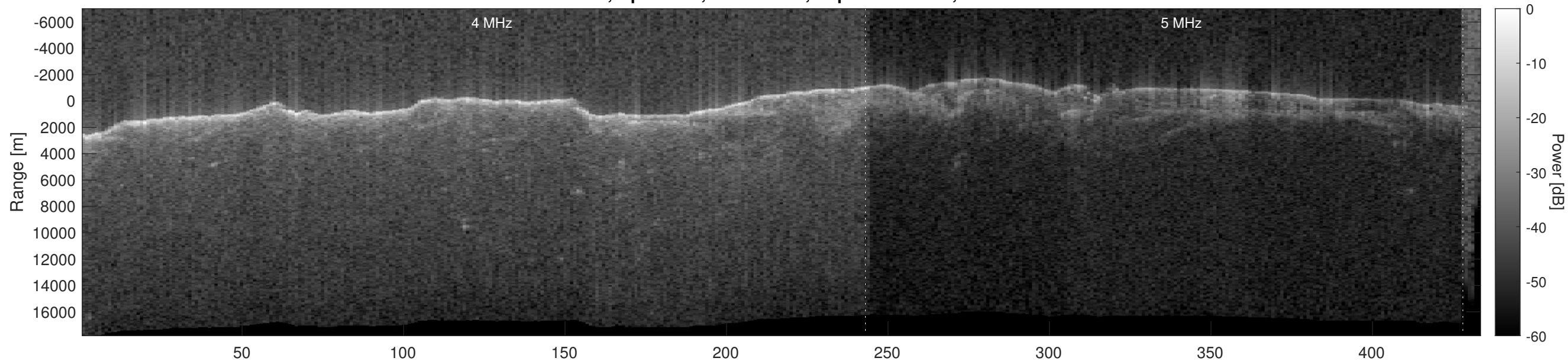
Orbit 21537, Optimized, No Window, Depth-Corrected, Channel 2
