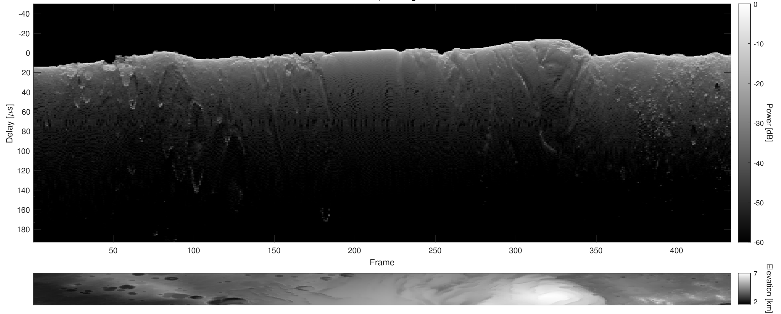
Orbit 21539, Cluttergram
