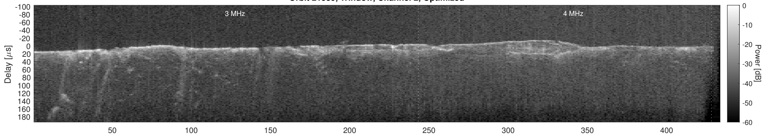
Orbit 21539, Cluttergram
