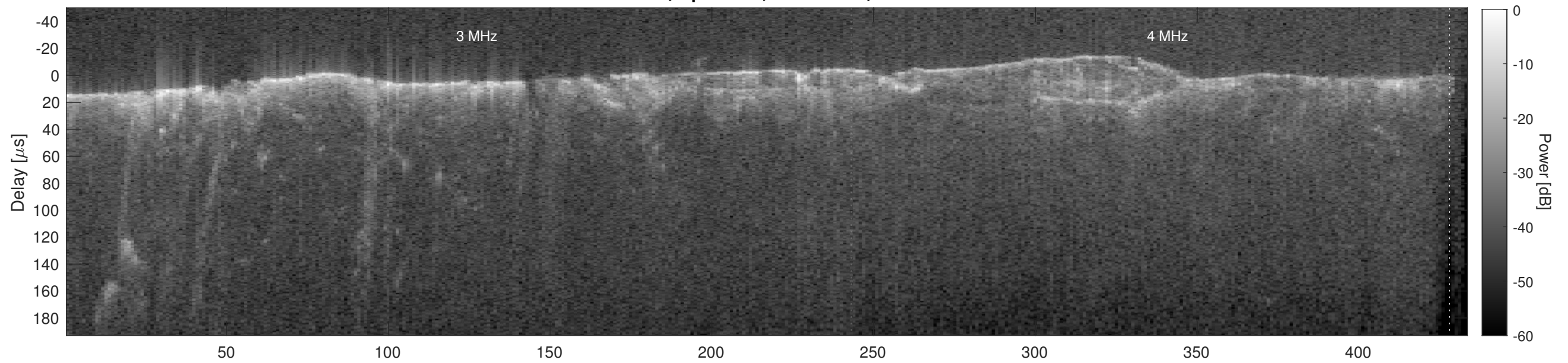
Orbit 21539, Cluttergram
