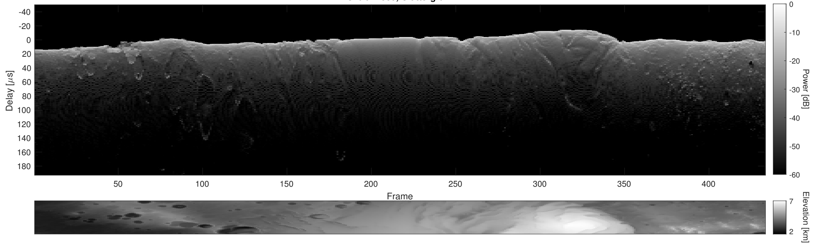
Orbit 21539, Cluttergram
