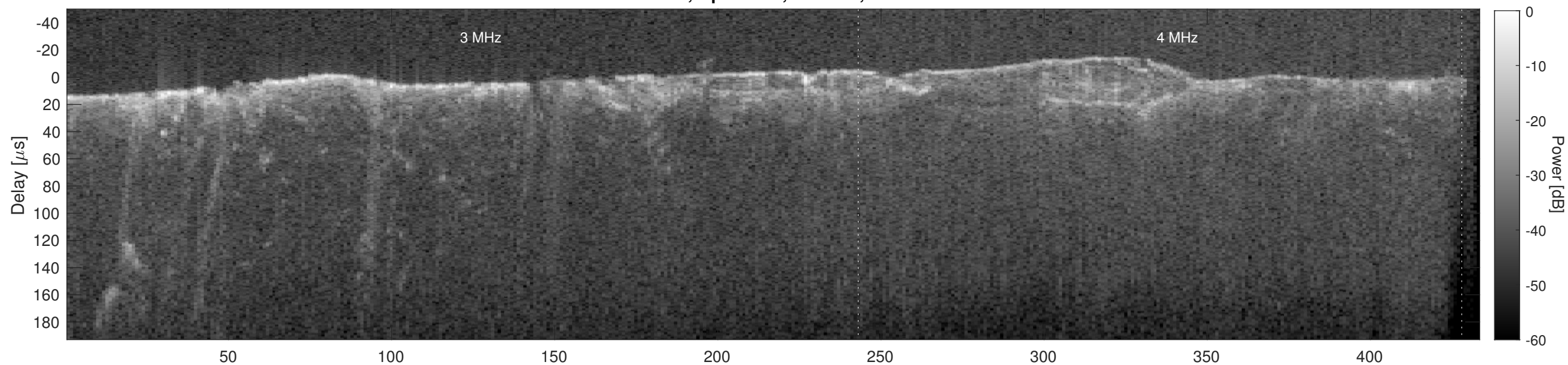
Orbit 21539, Cluttergram
