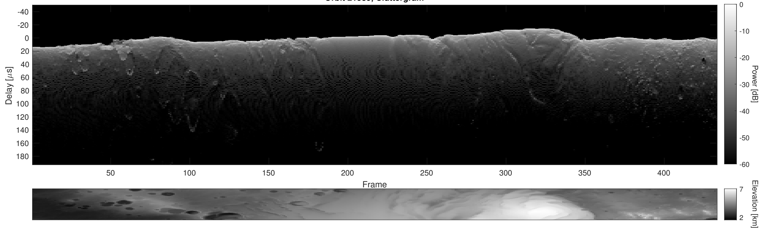
Orbit 21539, Cluttergram
